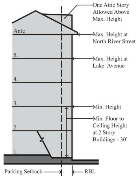
BUILDING TYPE 'B' - HEIGHT
